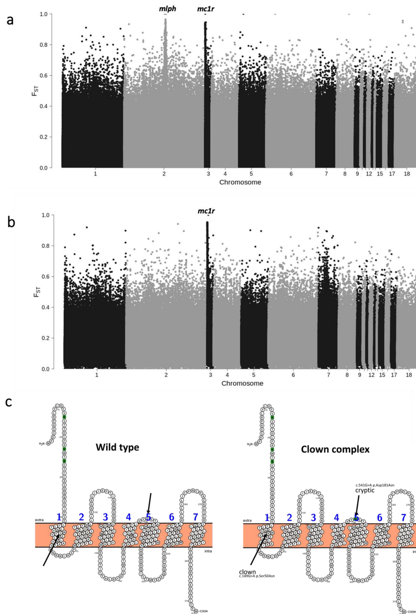
FIGURE 2 | (a) Manhattan plot ( Python_molurus_bivittatus-5.0.2_HiC assembly) of F_{ST} values for the Clown phenotype (case) against a reference pool (control). It was established through pedigree data that control samples do not have the Clown mutation, but they all carry the mutation responsible for the Hypo–Ghost colour morph. The candidate gene for Clown maps within the peak on Chromosome 3. The peak on Chromosome 2 contains the candidate gene ( mlph ) of the Hypo–Ghost colour morph (Lederer et al. 2023). (b) Manhattan plot of F_{ST} values between Clown ( n = 38 ) and Spider control pool ( n = 26 ). (c) On Chromosome 3, a missense mutation (p.Ser50Asn) in the protein coding region of the melanocortin-1 receptor ( mc1r ) gene is associated with the Clown phenotype. The putative Clown variant is located in the first transmembrane domain of mc1r . The candidate Cryptic missense variant (p.Asp181Asn) maps to the extracellular region between the fourth and fifth intracellular domains. The Clown and Cryptic loci are indicated by an arrow on the wild type and Clown complex models. The green square corresponds to the N-glyco motif.
